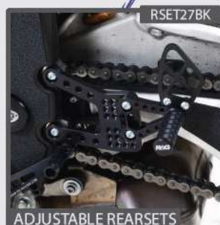
ADJUSTABLE REARSETS
